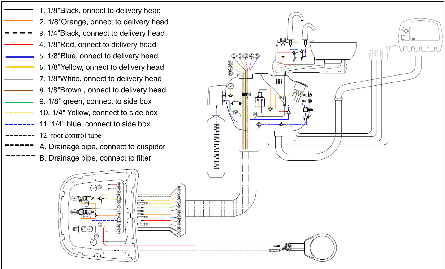
Figure 42 Beyond300, water unit
