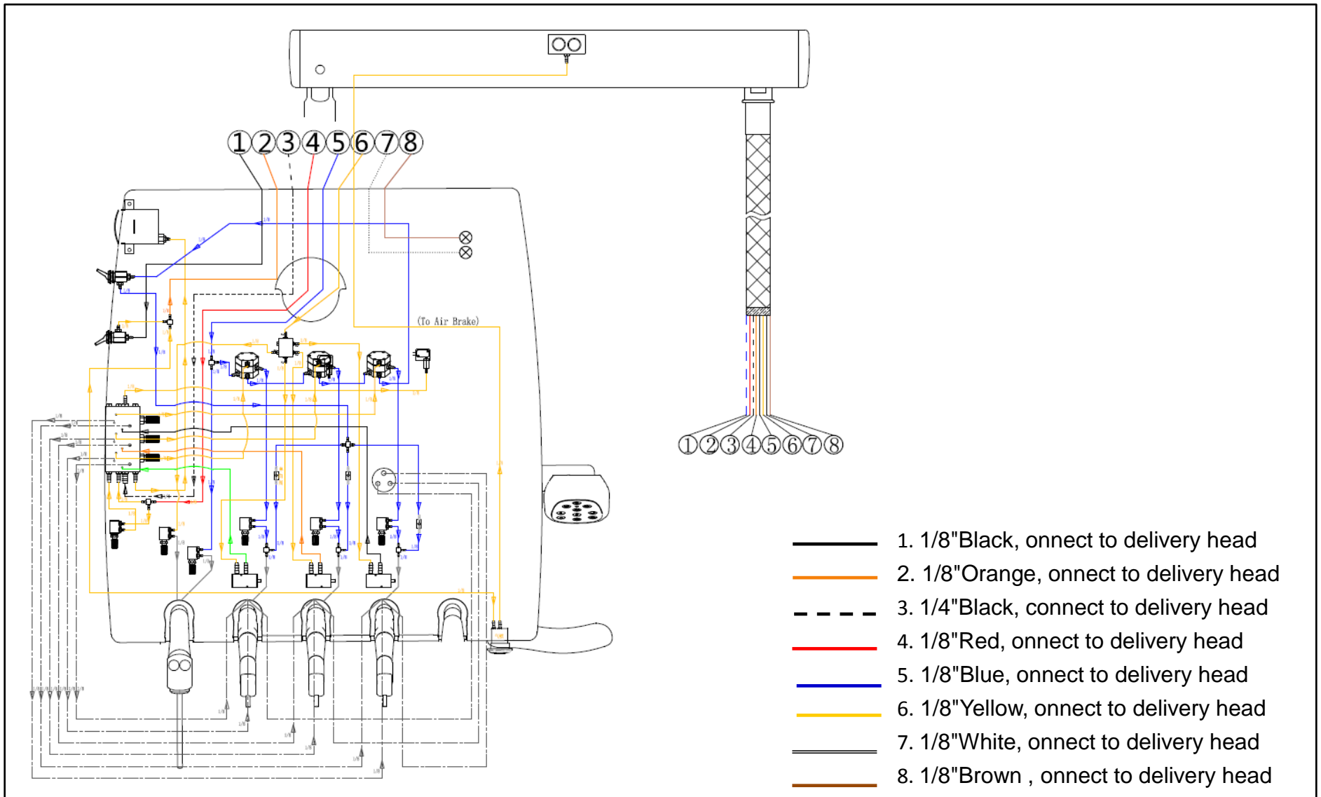
Figure 41 Beyond300, delivery head
