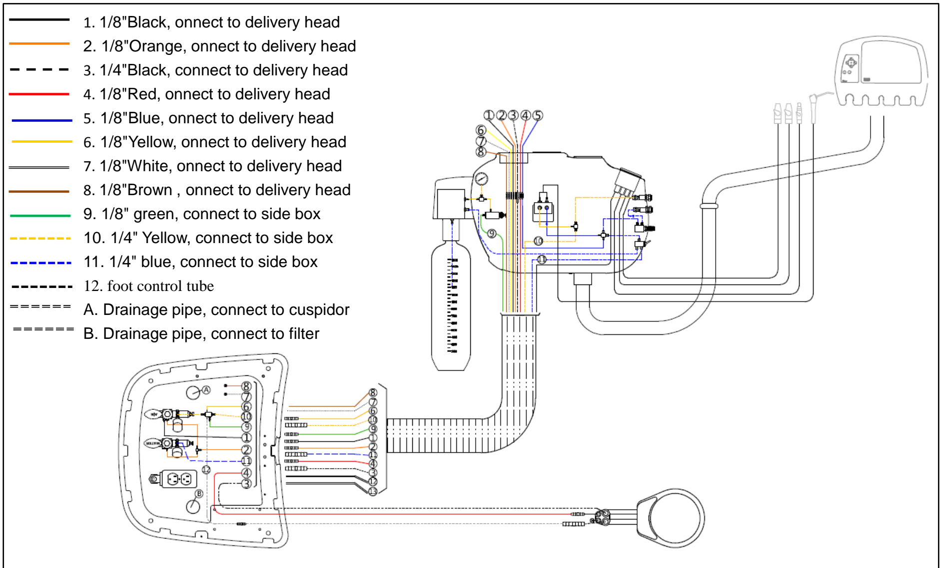
Figure 43 Beyond301, water unit
